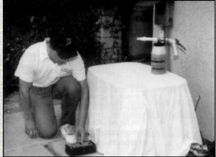
The cloth barrier prevents air dilution and refrigerant drift. Sensing probe is placed under the compressor.
